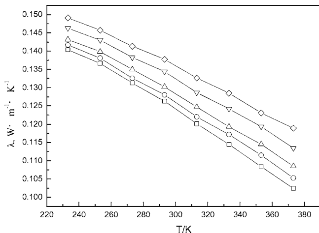
Figure 6. Temperature dependence of the thermal conductivity of dibutyl ether at different temperatures: \diamond , 30 MPa; \nabla , 20 MPa; \triangle , 10 MPa; \circ , 5 MPa; \square , 0.2 MPa.
