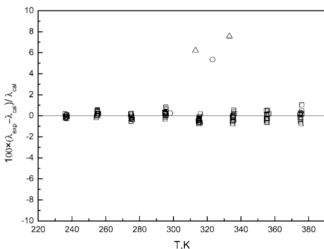
Figure 7. Relative deviations of calculated values by eq 1 from experimental data for pure dibutyl ether: \square , this work; \circ , ref 9; \triangle , ref 10.
